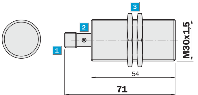
Dimensional drawing
