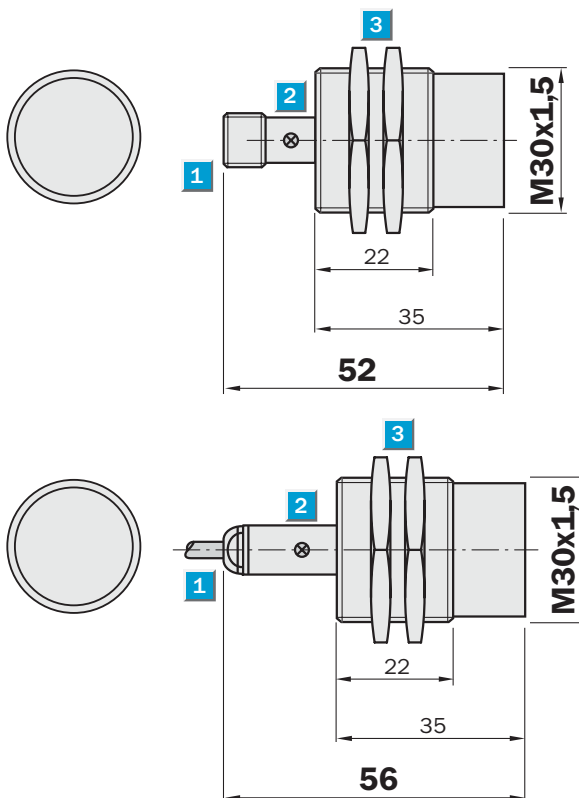
Dimensional drawing
